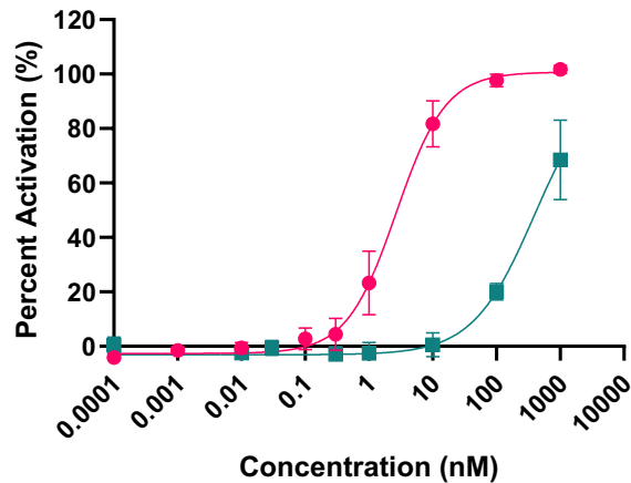
MC3R selective
