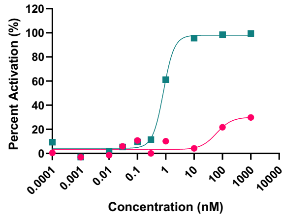
MC4R selective
